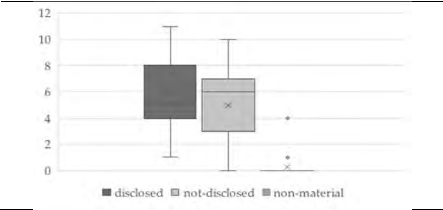
Figure 3 – Boxplots of the employee dimension
