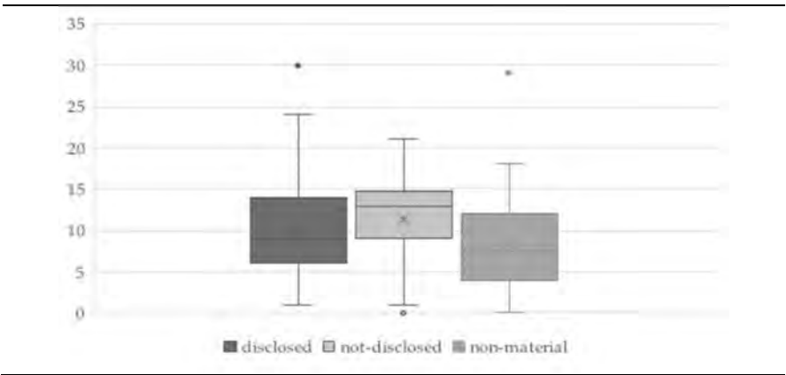
Figure 1 – Boxplots of the environmental dimension
