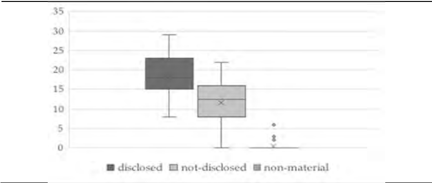
Figure 8 – Boxplots of the policies
