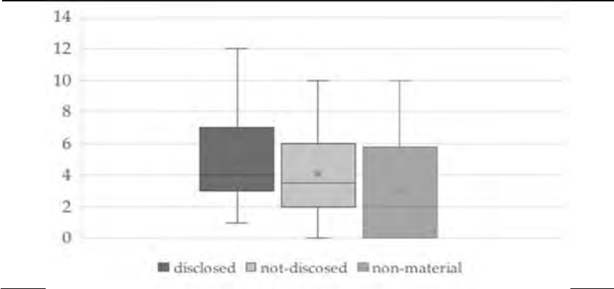
Figure 2 – Boxplots of the social dimension
