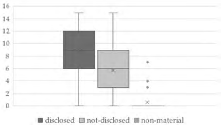
Figure 9 – Boxplots of risks and opportunities
