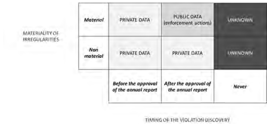
Figure 2 – Misreporting and data availability
