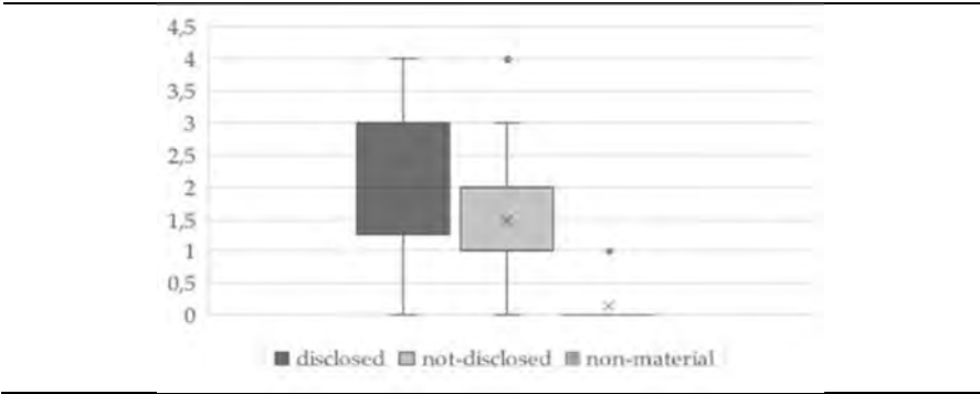
Figure 6 – Boxplots of the gender diversity dimension
