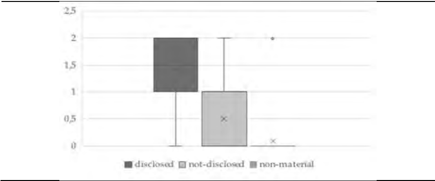
Figure 6 – Boxplots of the gender diversity dimension
